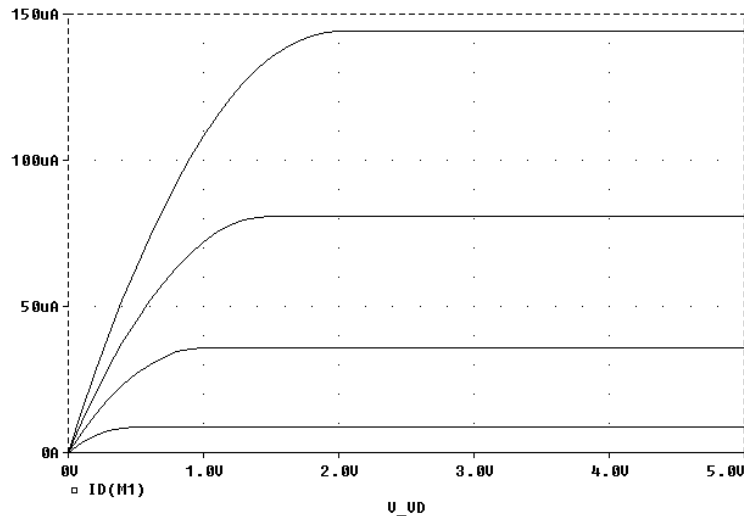
Figure 9-3 Device curve family.
