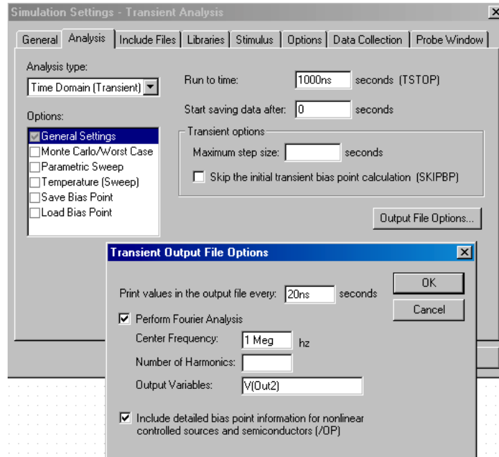
Figure 12-1 Transient analysis setup for EXAMPLE.OPJ.
