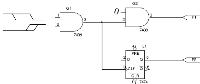
Figure 14-3 Circuit with a timing ambiguity
