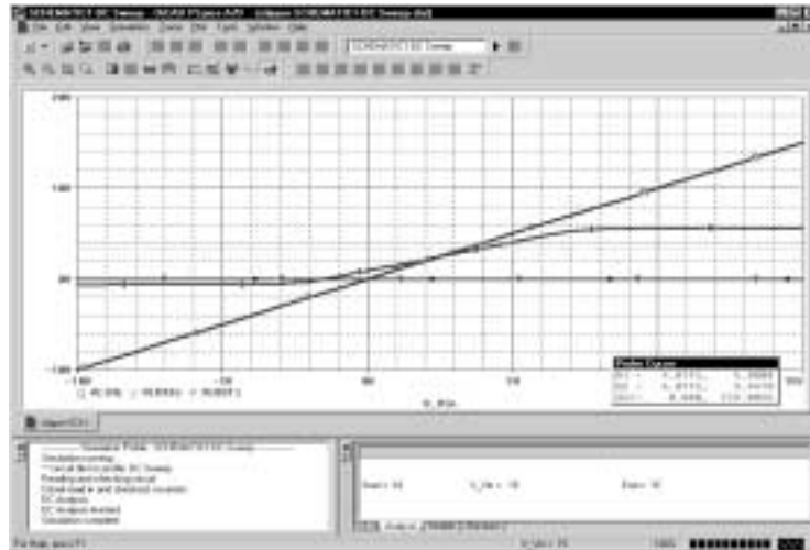
Figure 2-12 Voltage difference at V(In) = 4 volts.
