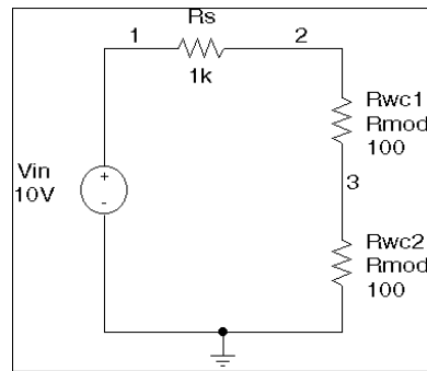
Figure 13-17 Schematic using VARY BOTH.
