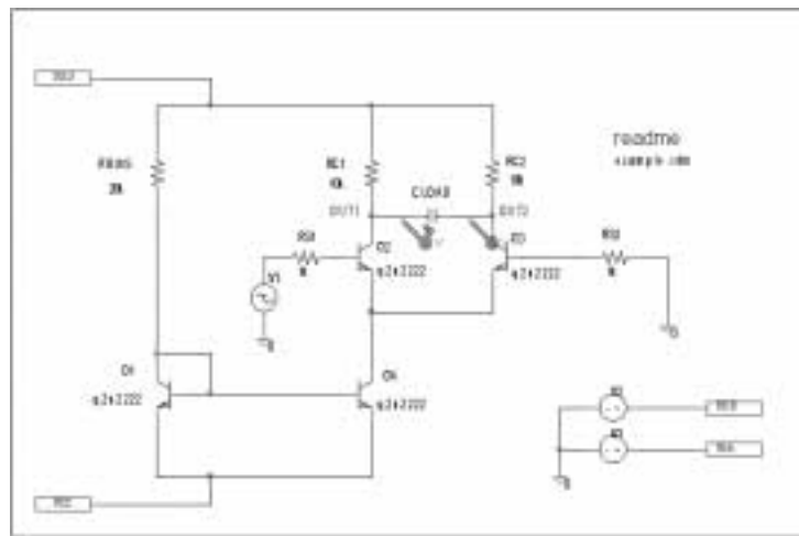
Figure 13-1 Example schematic EXAMPLE.OPJ.
