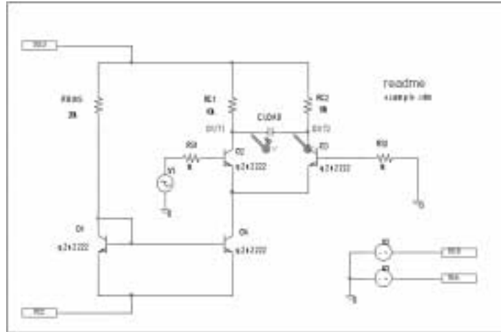
Figure 12-2 Example schematic EXAMPLE.OPJ.
