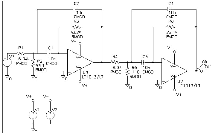
Figure 13-8 Chebyshev filter.
