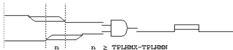
Figure 16-13 Glitch suppression example one.
