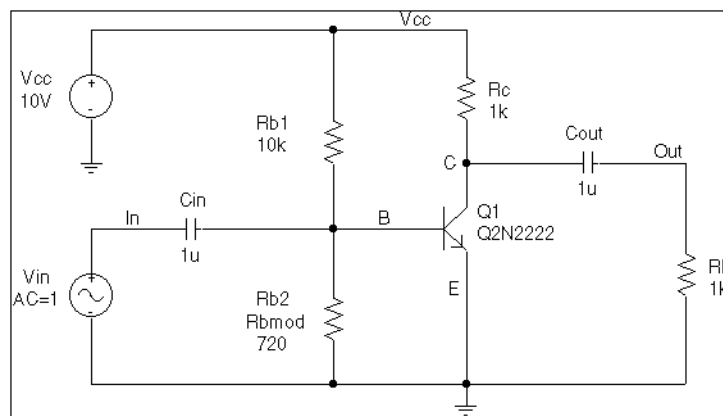
Figure 13-11 Simple biased BJT amplifier.
