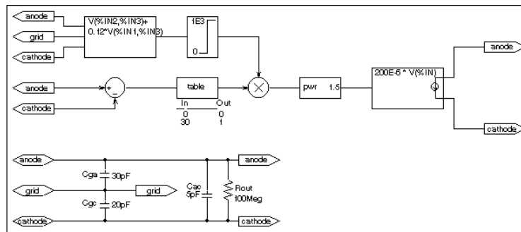
Figure 6-13 Triode circuit.
