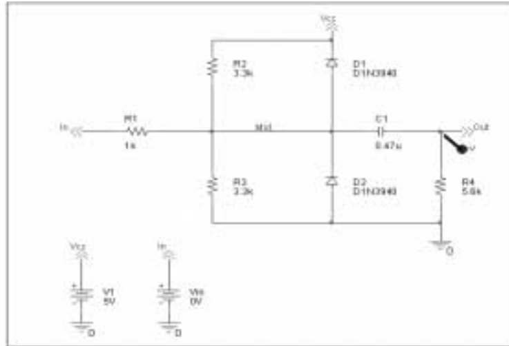
Figure 2-8 Clipper circuit with voltage marker on n Out.
