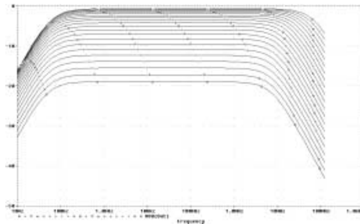
Figure 2-23 Small signal response as R1 is varied from 100 \Omega to 10 k \Omega .
