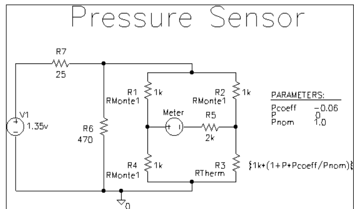
Figure 13-7 Pressure sensor circuit with RMonte1 and RTherm model definitions.
