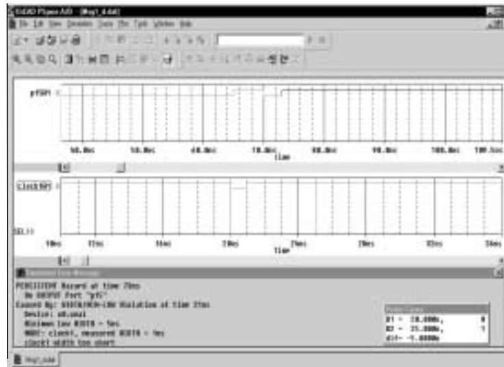
Figure 17-11 Waveform display for a persistent hazard.
