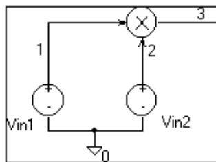
Figure 6-20 Voltage multiplier circuit (mixer).
