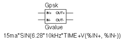
Figure 6-16 GVALUE part example.
