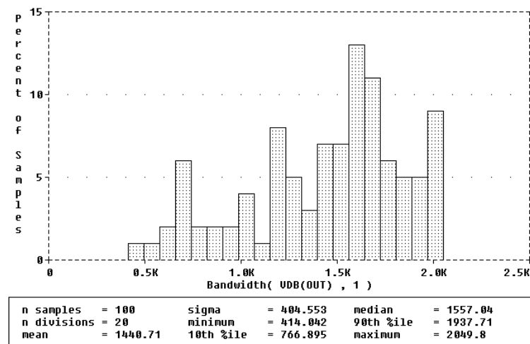
Figure 13-9 1 dB bandwidth histogram.
