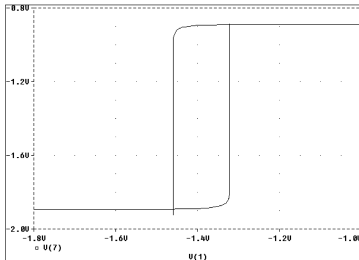
Figure 12-5 Hysteresis curve example: Schmitt trigger.
