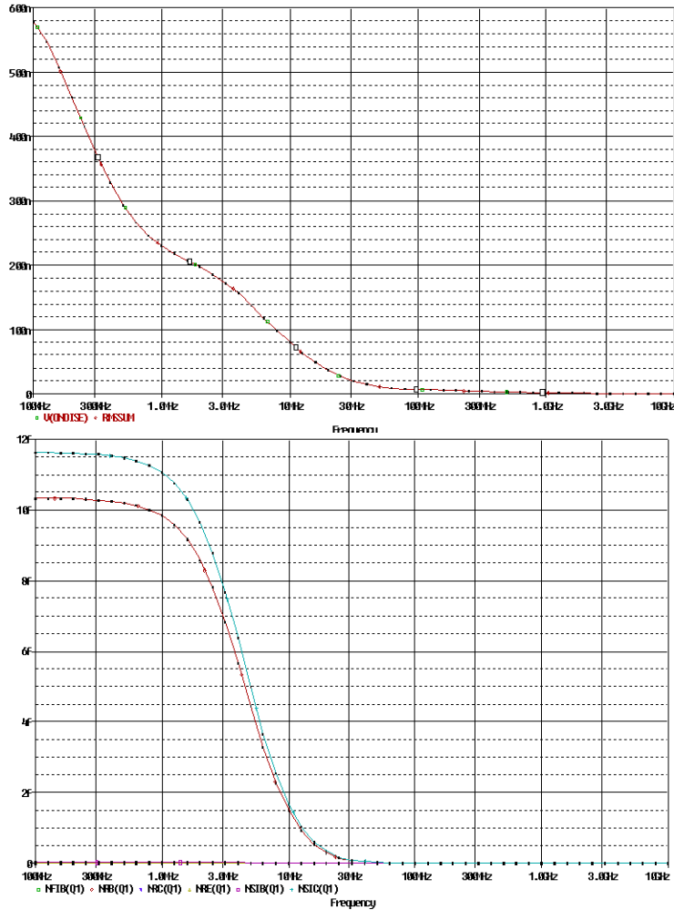
Figure 10-3 Device and total noise traces for EXAMPLE.OPJ.
