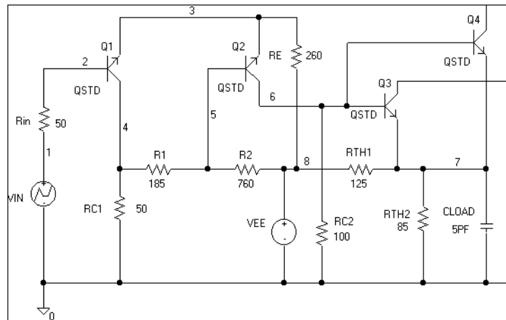
Figure 12-3 ECL-compatible Schmitt trigger.
