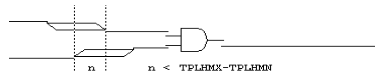
Figure 16-14 Glitch suppression example two.
