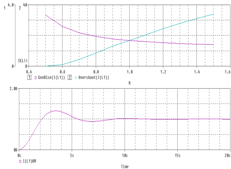
Figure 11-3 Rise time and overshoot vs. damping resistance.
