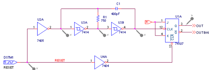
Figure 17-7 Mixed analog/digital oscillator
