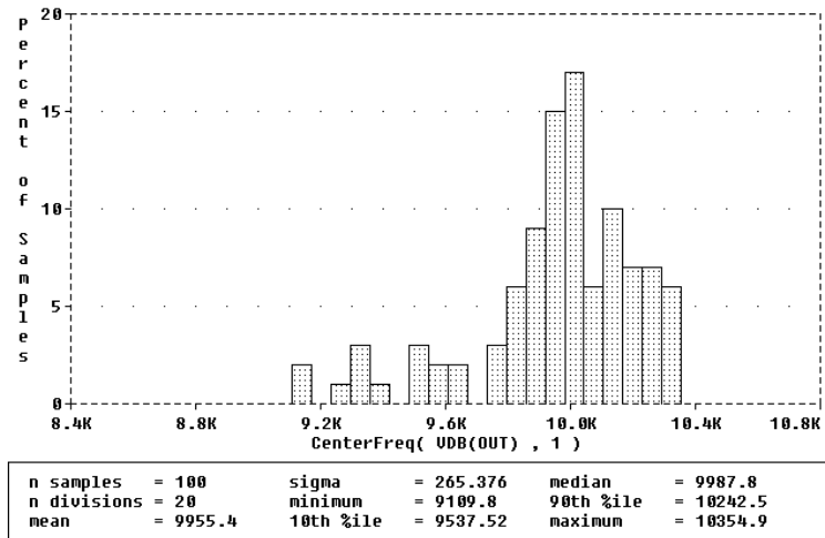
Figure 13-10 Center frequency histogram.
