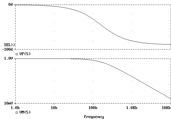
Figure 6-7 Viewing gain and phase characteristics of a lossy integrator.
