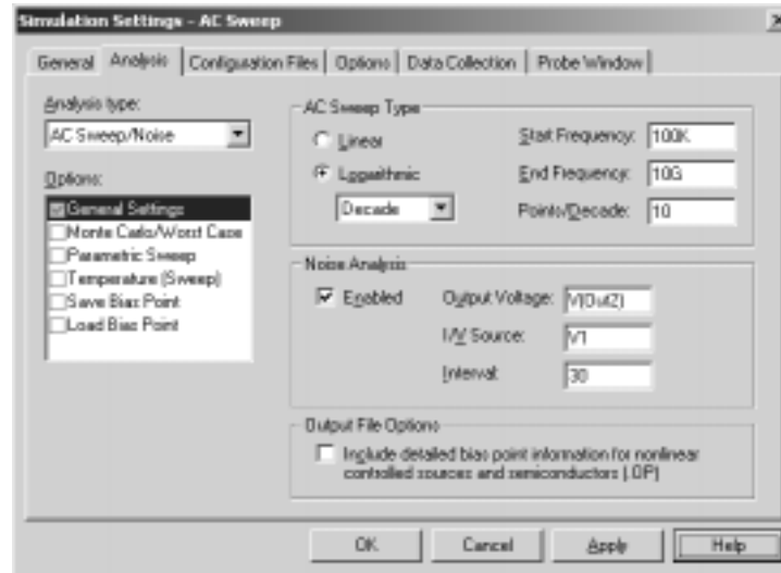
Figure 10-2 AC analysis setup for EXAMPLE.OPJ.
