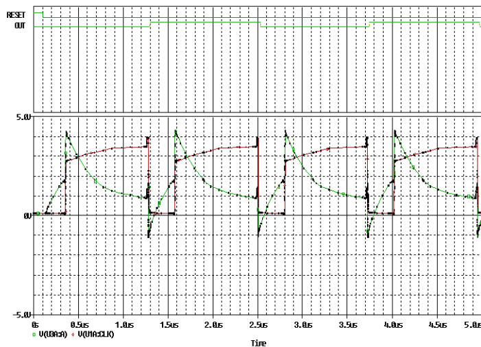
Figure 17-9 Mixed analog/digital oscillator results.
