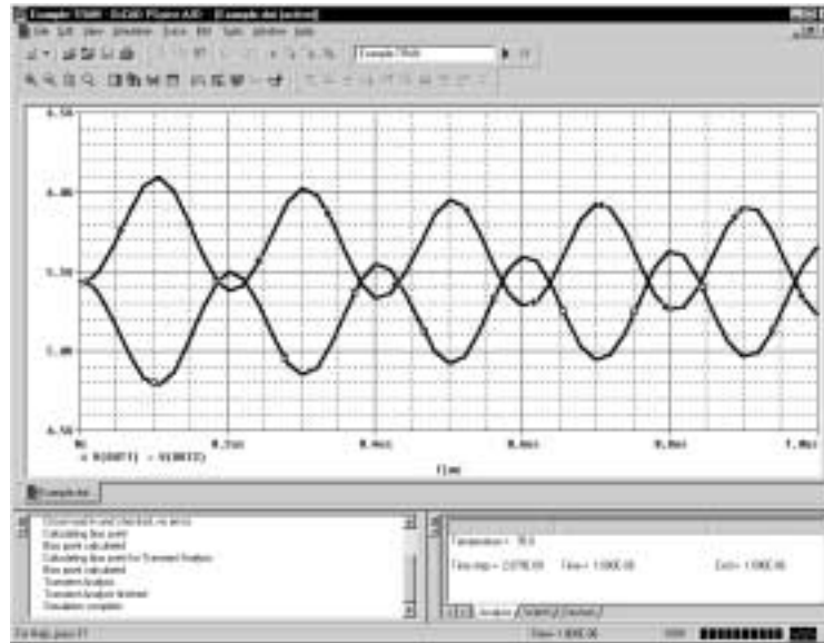
Figure 17-6 Waveform display for EXAMPLE.DAT .
