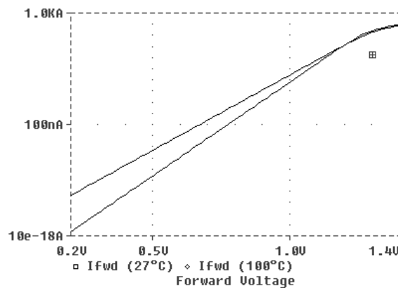
Figure 4-7 Forward Current device curve at two temperatures.
