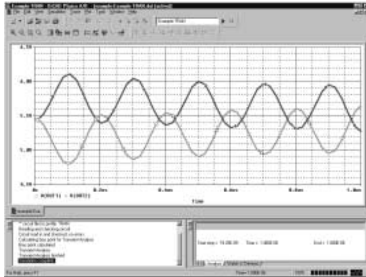
Figure 8-1 PSpice simulation window
