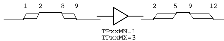
Figure 16-8 Cumulative ambiguity hazard example one.
