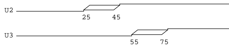
Figure 16-12 Reconvergence hazard example two.
