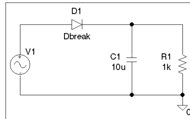
Figure 4-4 Design for a half-wave rectifier.
