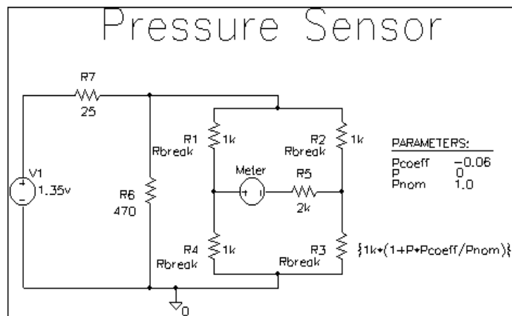
Figure 13-5 Pressure sensor circuit.
